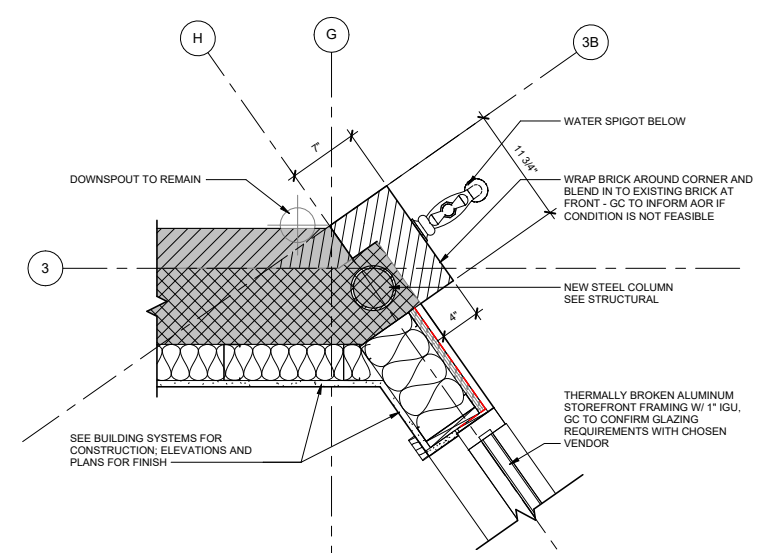
OLD TO NEW TRANSITION DETAIL
