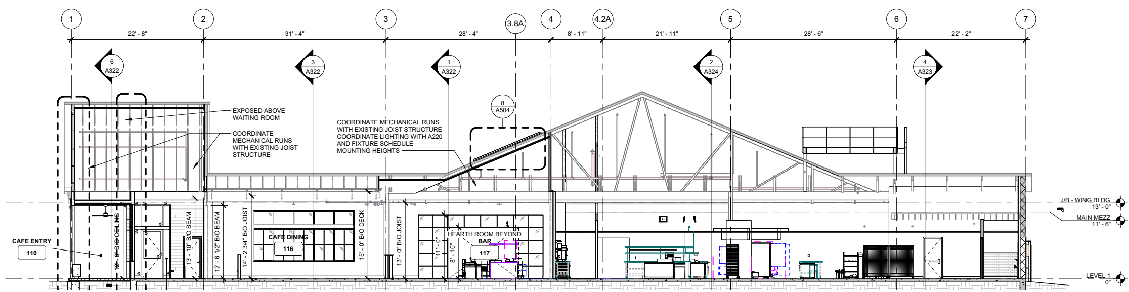
TECHNICAL SECTION
