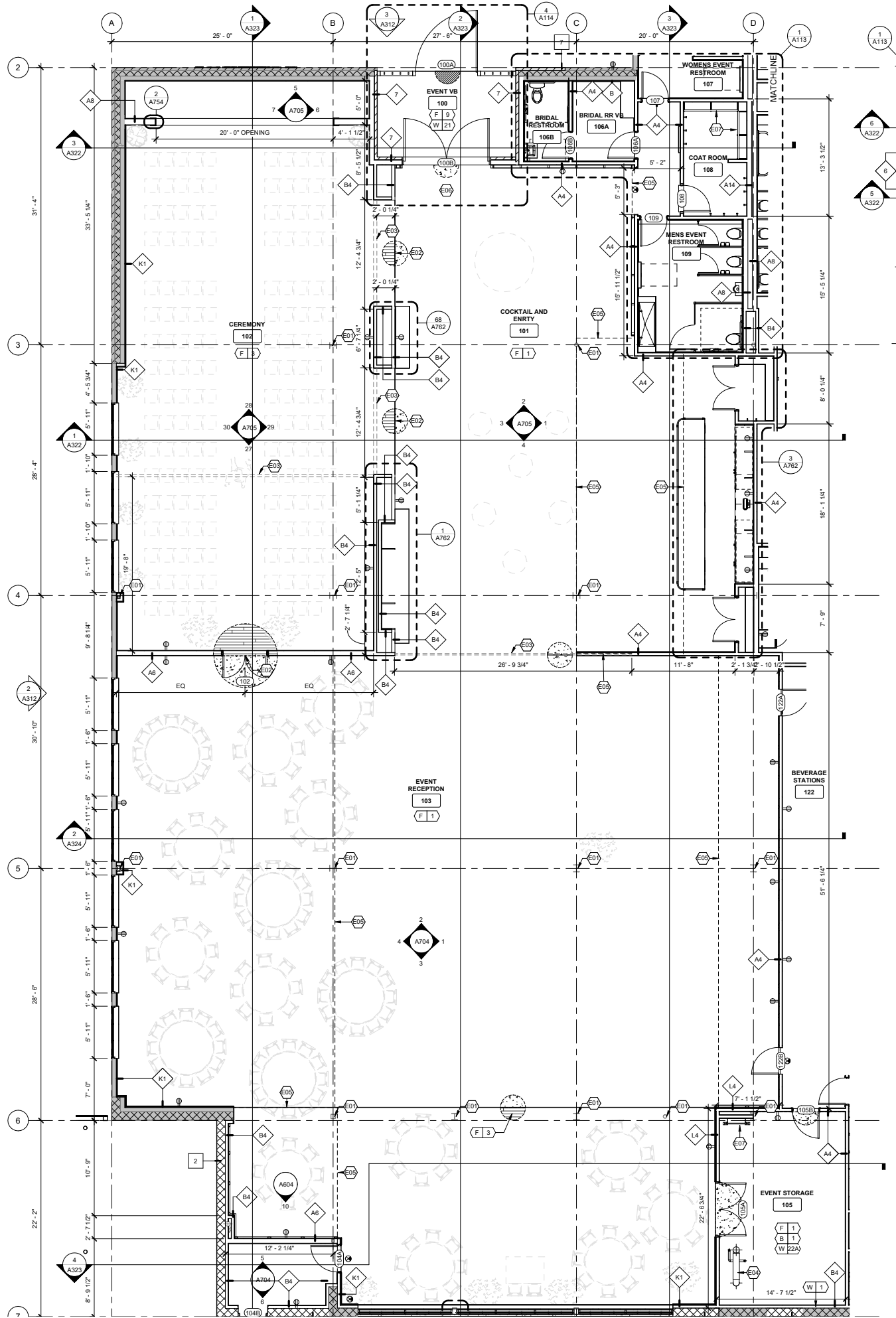
EVENTS FLOOR PLAN
