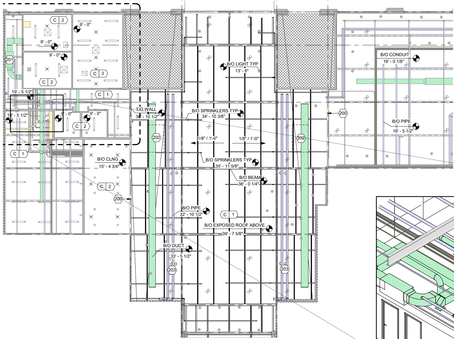
SURVEY REFLECTED CEILING PLAN
