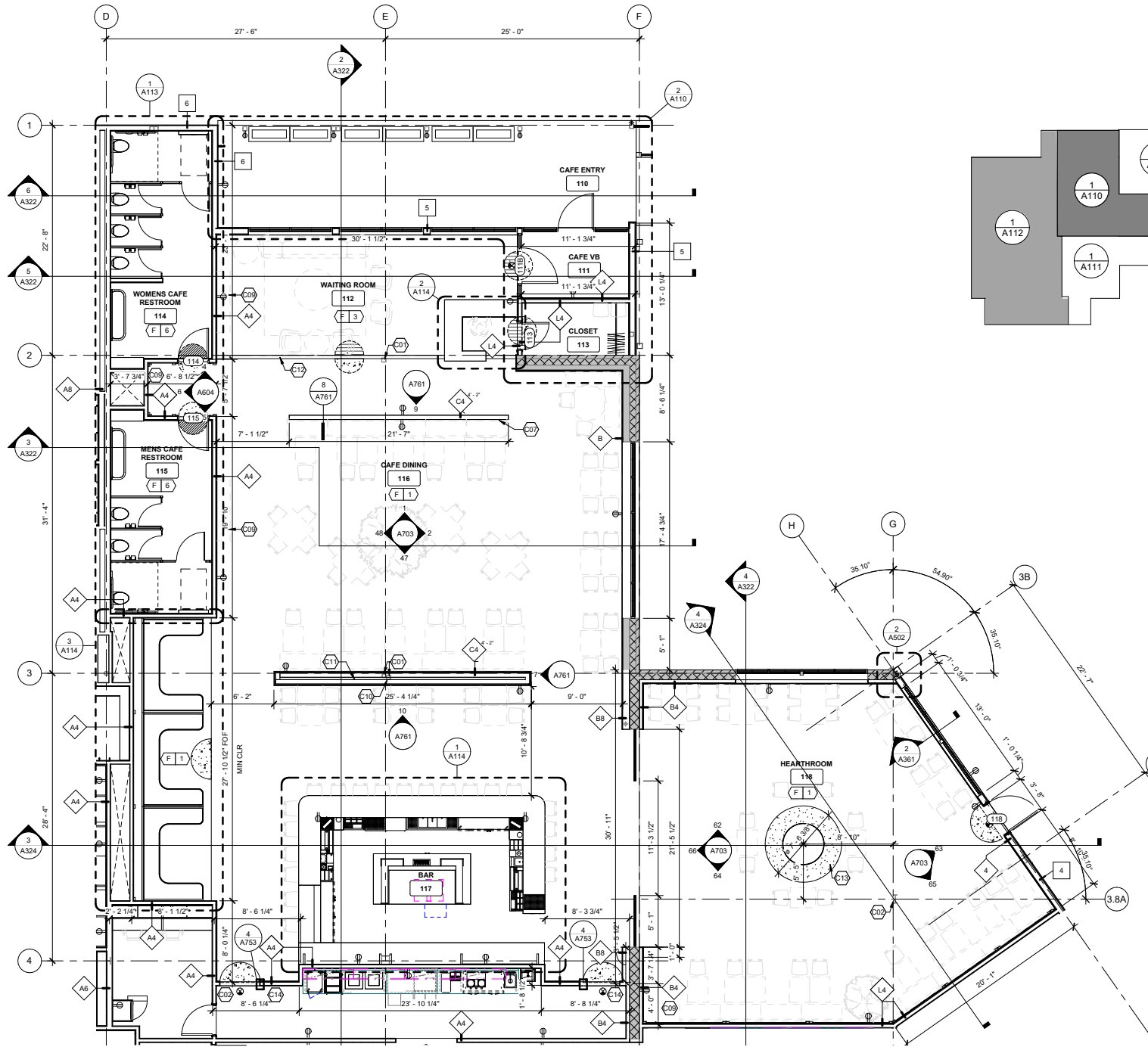
CAFE FLOOR PLAN
